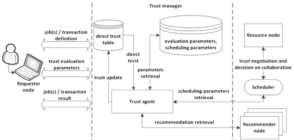
Figure 2: Trust manager architecture from the requester's point of view.
