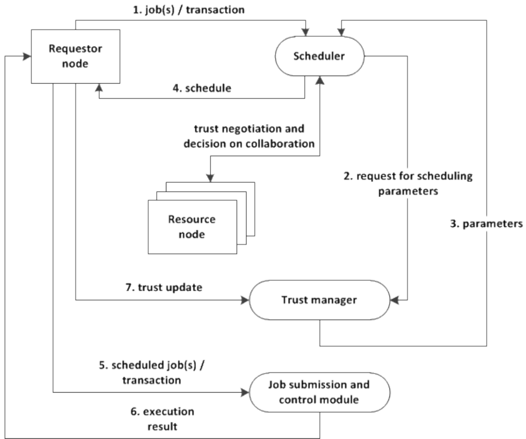
Figure 1: Trust manager integration into the ad hoc grid infrastructure from the requester's point of view.
