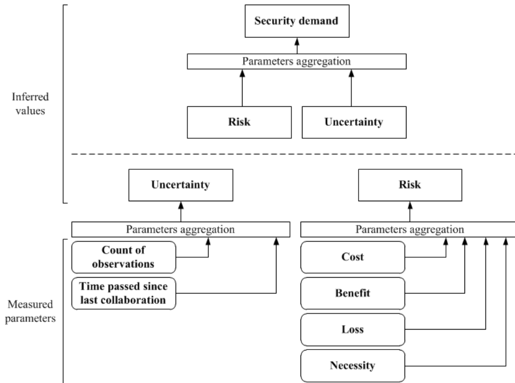
Figure 4: Security demand inferred from trust components.
