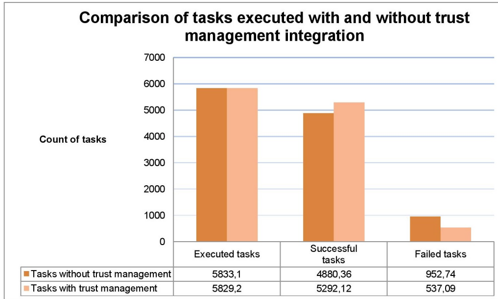
Figure 6: Comparison of tasks executed with and without trust management integration into the modelled ad hoc grid infrastructure.
