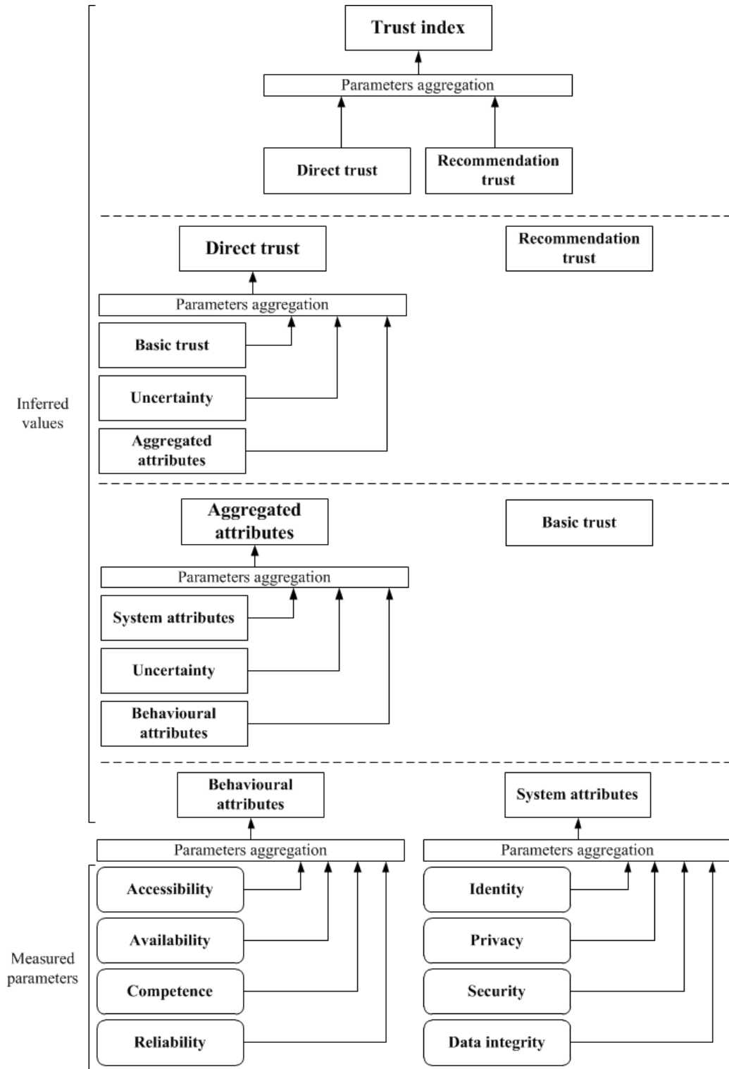
Figure 5: Trust index inferred from trust components.
