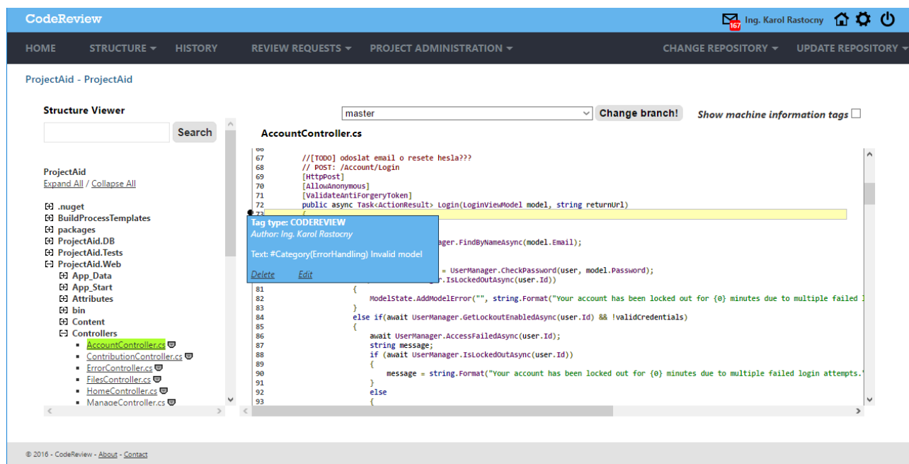
Figure 2: System CodeReview, displaying one source code file with information tag.
