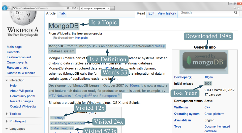
Figure 1: Examples of simple information tags in a human-readable format. An arrow and a highlighted text represent anchoring, the first word defines a type and the second word represents a body of an information tag.
