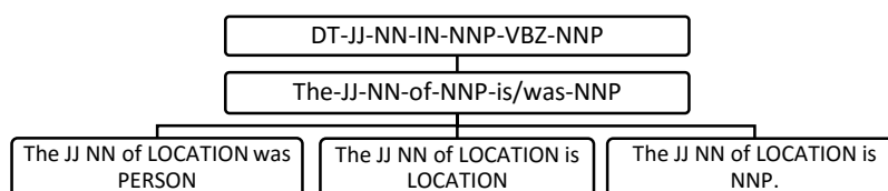
Figure 1: Hierarchy of sentence patterns based on level of abstraction [4].
