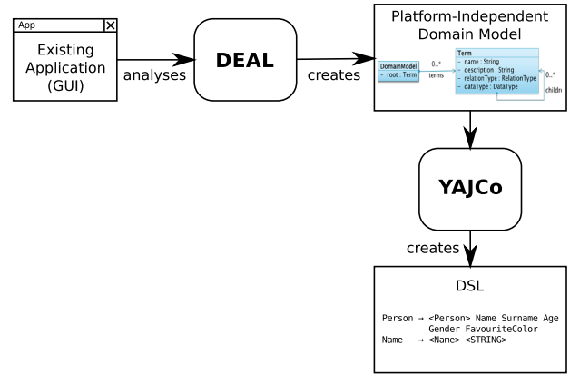
Figure 1: The concept of the DEAL method for domain language extraction
