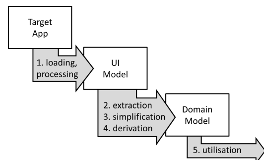
Figure 2: Phases of the DEAL method
